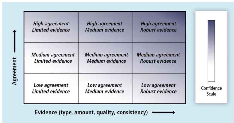
Levels of evidence and agreement contributing to a key finding (Source: IPCC)
